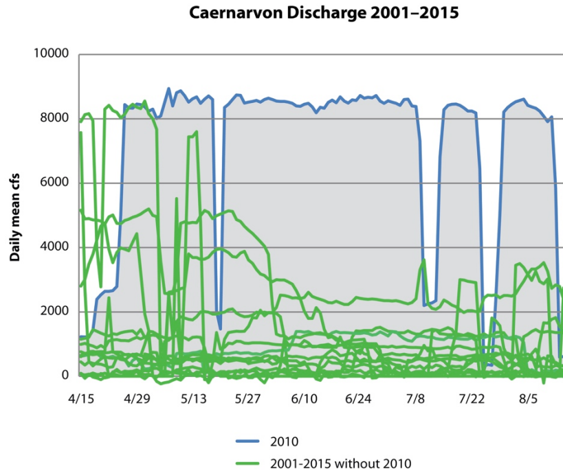
Figure 2.3-7. Highly atypical flow of fresh water discharged from the Caernarvon salinity control structure during the 2010 spill response (blue line), compared to daily water flow during the summer of years 2001–2015 (green lines).
